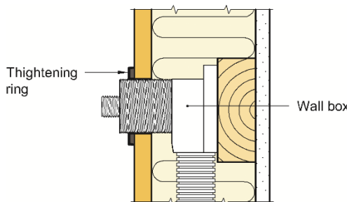
Fig. 4 Pipe penetration with tightening ring
